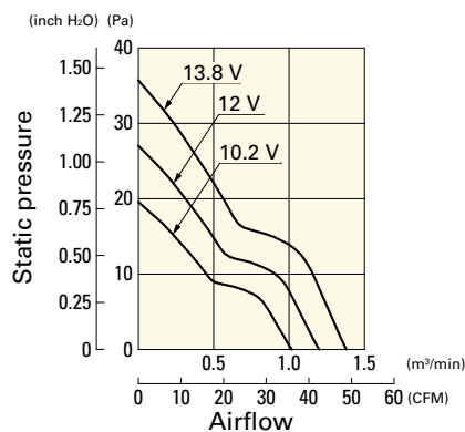
9G0924H201 With pulse sensor
